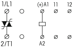
Connection diagram
