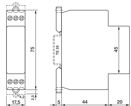
fig. 2. Dimensions (mm)
