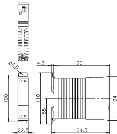
fig. 2. Dimensions (mm)
