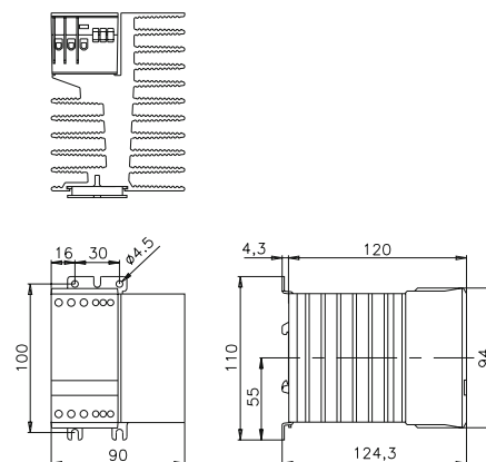
fig. 2. Dimensions (mm)
