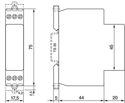
fig. 2. Dimension (mm)
