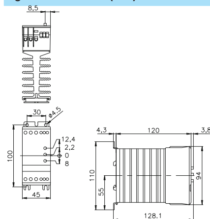
fig. 2. Dimensions (mm)
