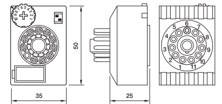
fig. 2. Dimensions (mm)
