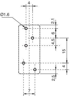
Printed circuit lay-out [mm]
