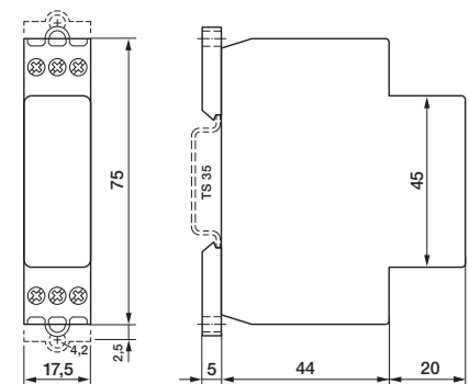
fig. 2. Dimensions (mm)
