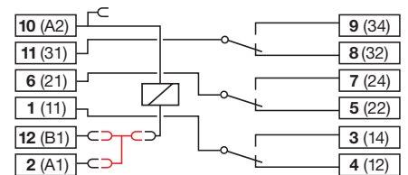
Connection diagram S3-MB1
