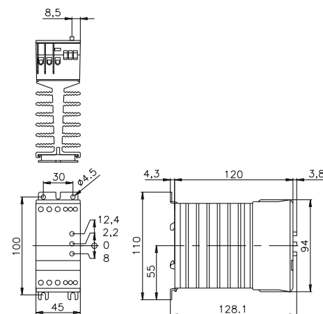
fig. 2. Dimensions (mm)
