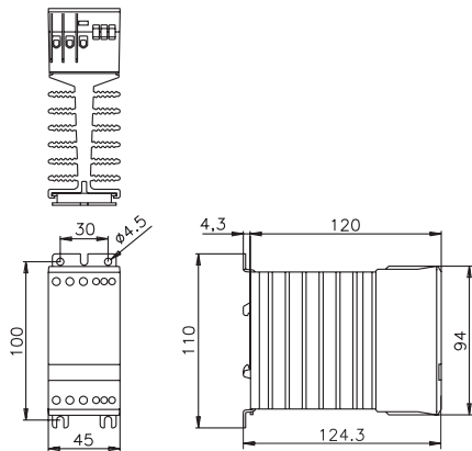
fig. 2. Dimensions (mm)
