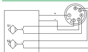
Mating Cordset: RKC 6T-*
