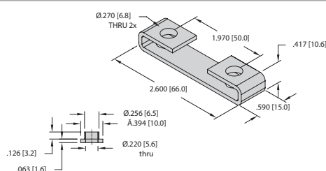
M5-Q25L
