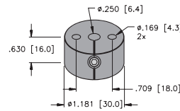
Positioning Element P2-Ri-QR14
