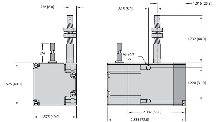
Dimensions: DW2000-55-**-C
