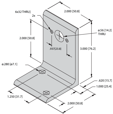
Magnet Mounting Bracket MMB-R10
