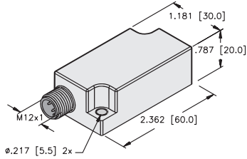
Q20L60 Housing
