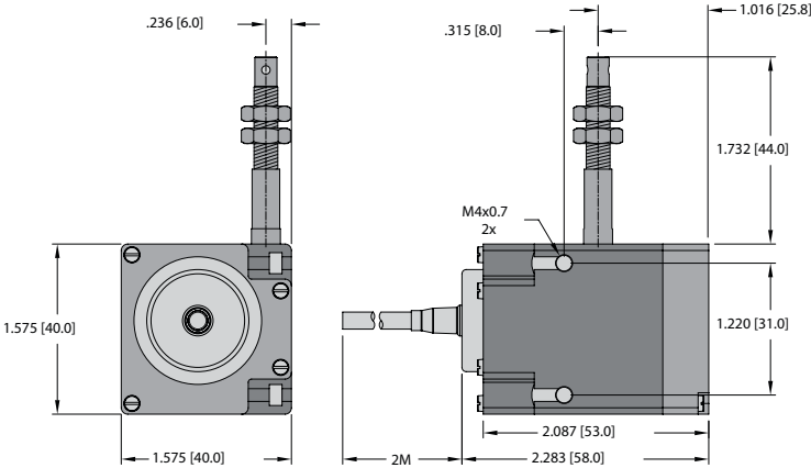
Dimensions: DW1000-55-**-CA
