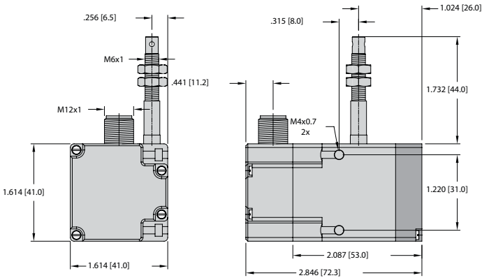
Dimensions: DW2000-55-**-H1141
