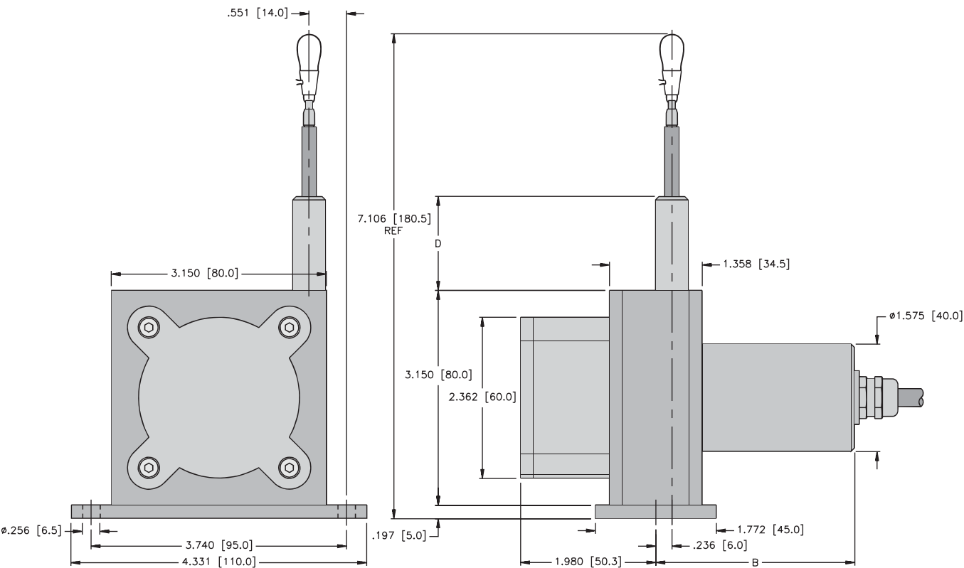
Dimensions: DW110 with Analog Sensor
