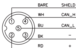
5-pin M12 Eurofast Connection
