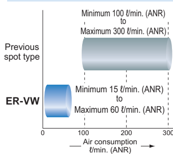
Comparison of air consumption
