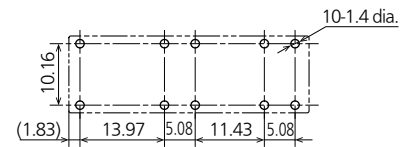
Recommended PC board pattern ( BOTTOM VIEW )
