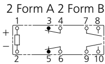
Schematic ( BOTTOM VIEW ) Standard
