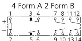
Schematic ( BOTTOM VIEW ) Standard
