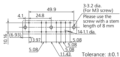
Recommended PC board pattern ( BOTTOM VIEW )
