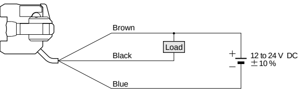
Wiring diagram
