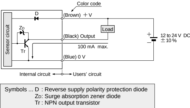
I/O circuit diagram
