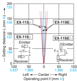
EX-11S□ / EX-11SE□
