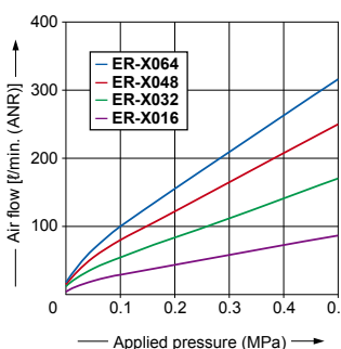
Air flow
