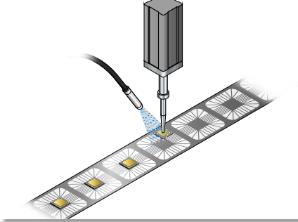
Preventing electrostatic damage during bonding
