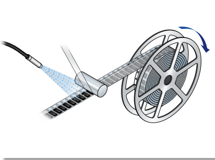
High-speed charge removal on a taping machine
