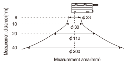
Measurement distance - Measurement area (typical)
