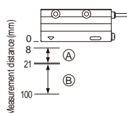
Range for measurement distance
