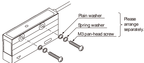
Example of recommended mounting
