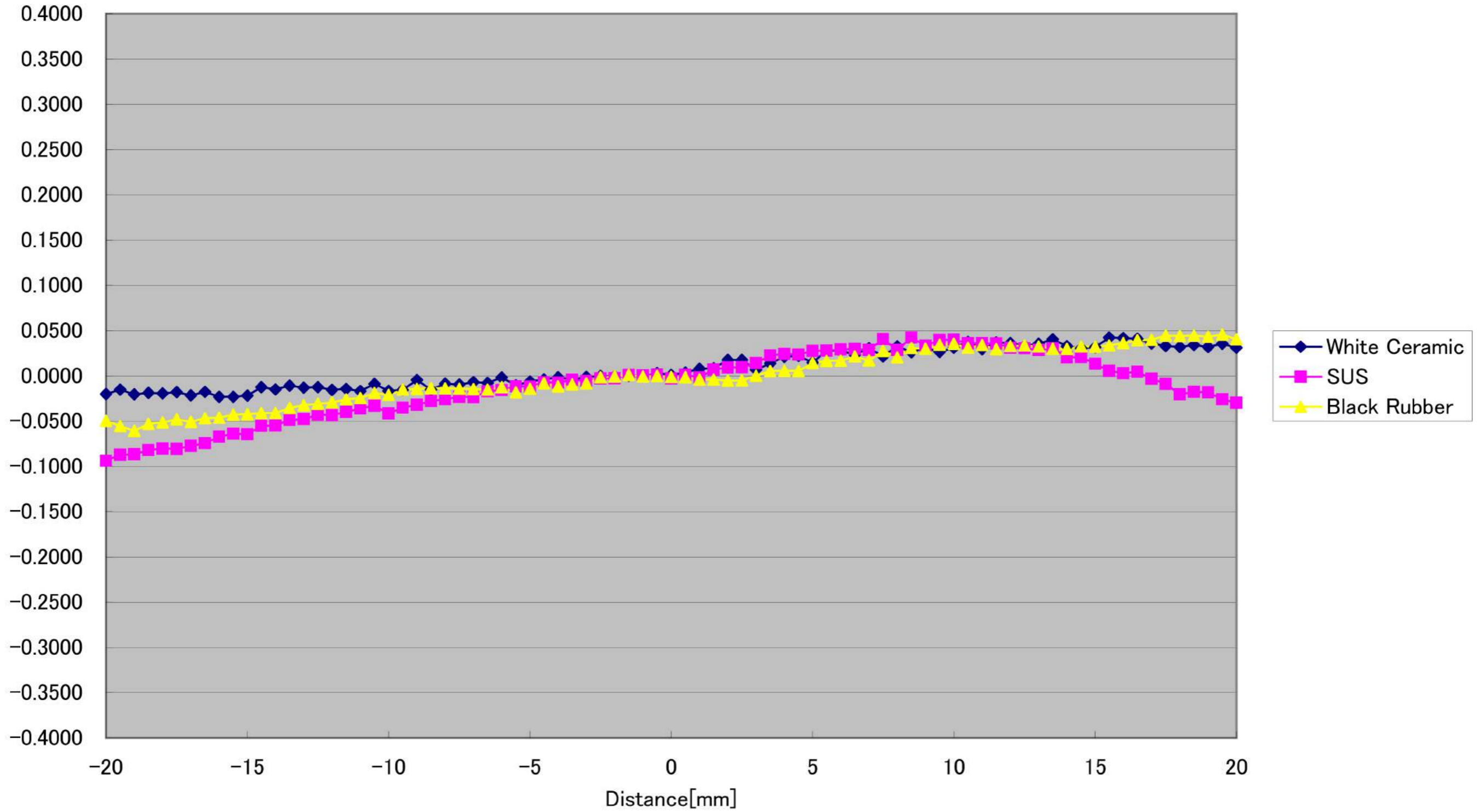
CD5-85-WIDE Linearity(Vertical -10^\circ )[%FS] (Typical)
