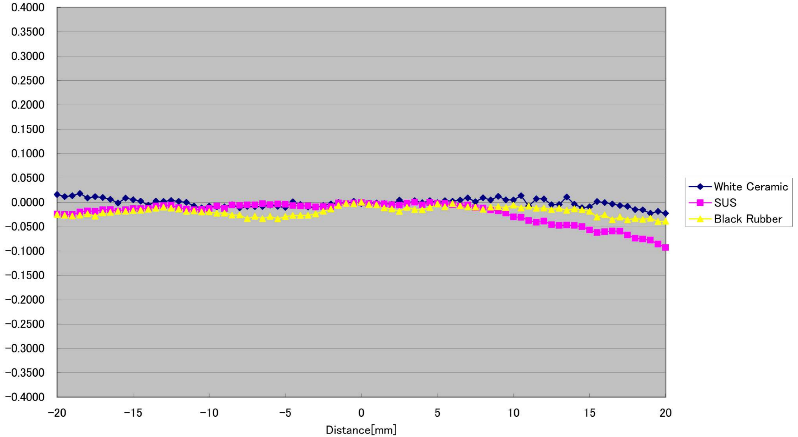
CD5-85-WIDE Linearity(Horizontal 10° )[%FS] (Typical)
