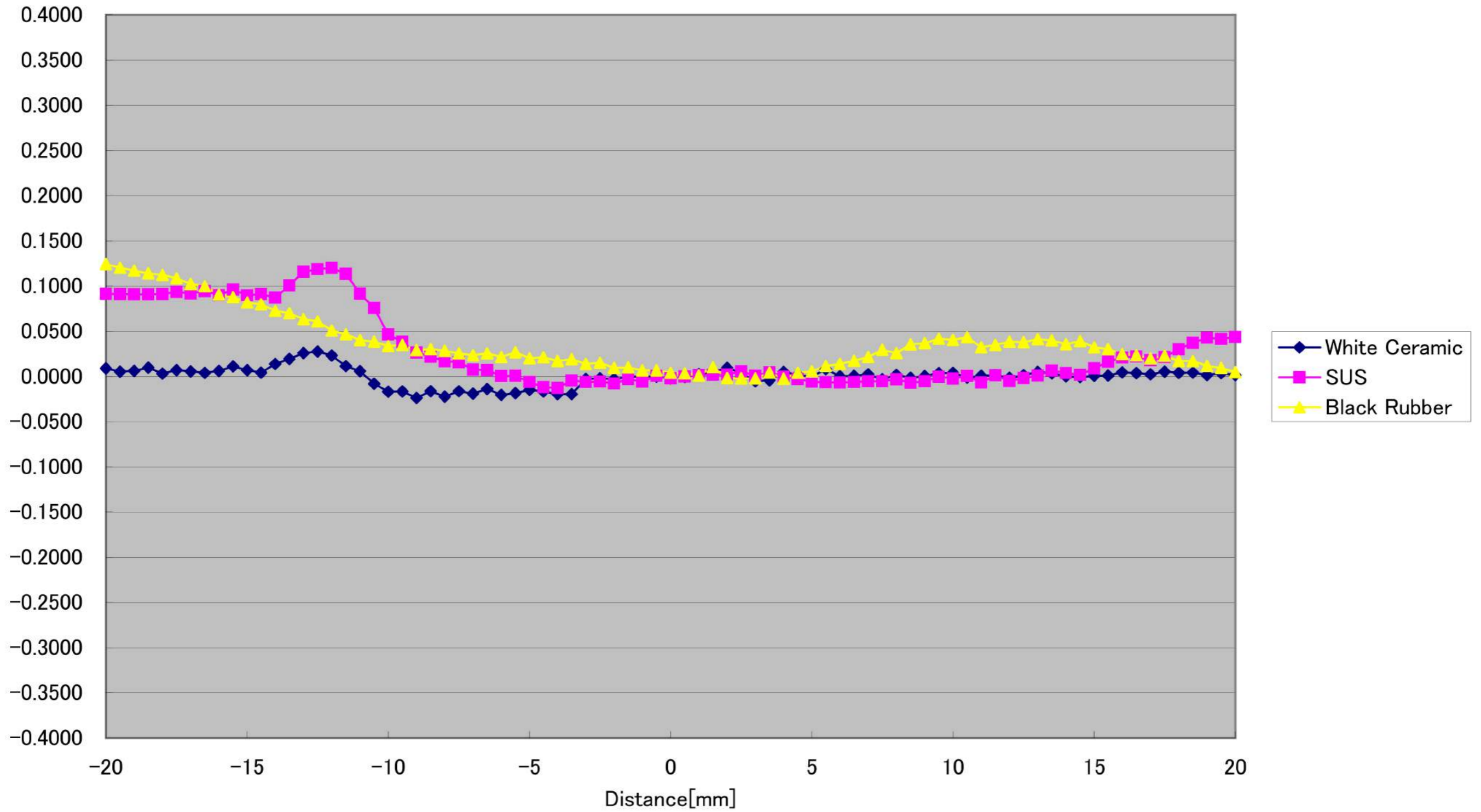
CD5-85-WIDE Linearity(Vertical +10° )[%FS] (Typical)
