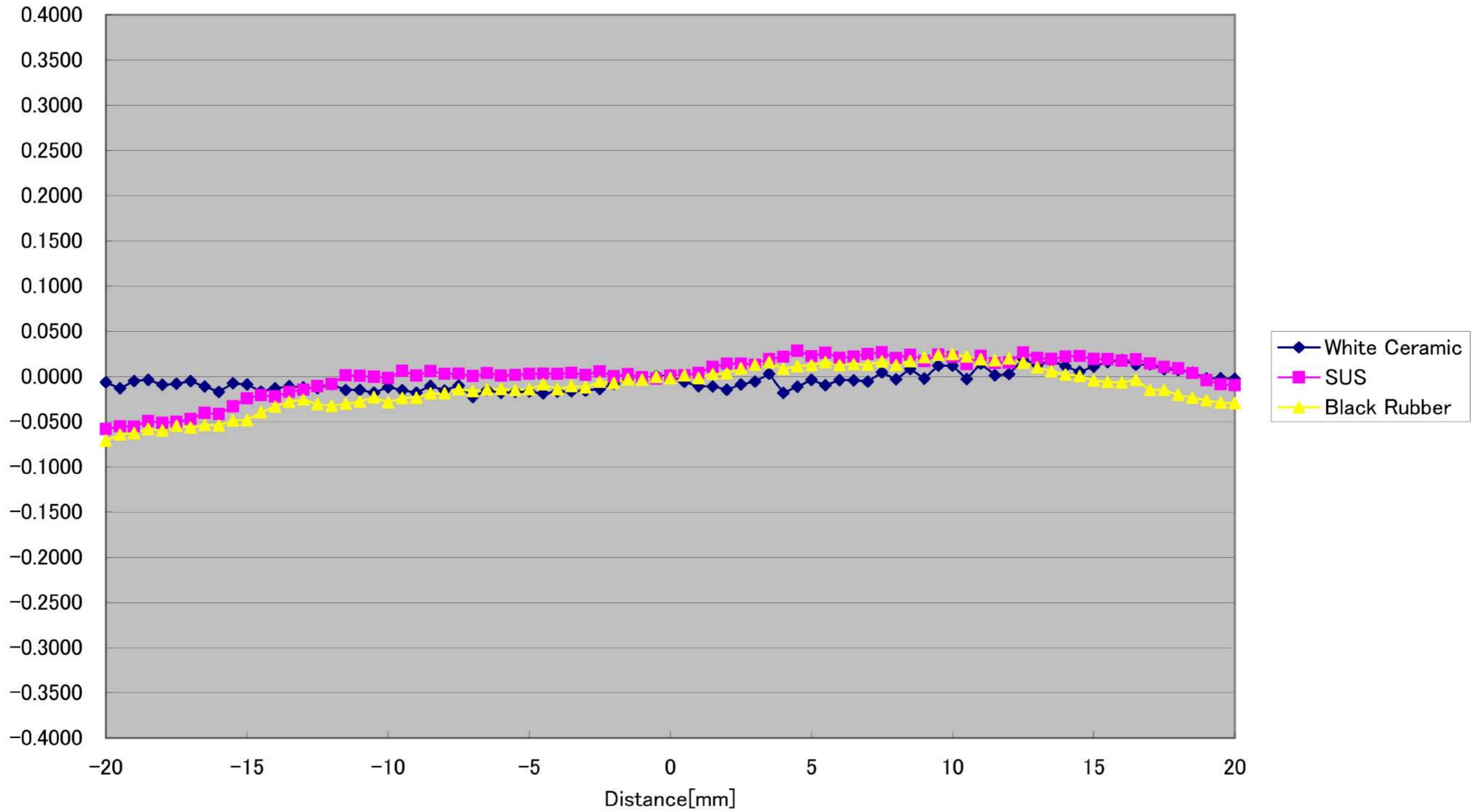
CD5-85-WIDE Linearity( \pm 0^\circ ) [%FS] (Typical)
