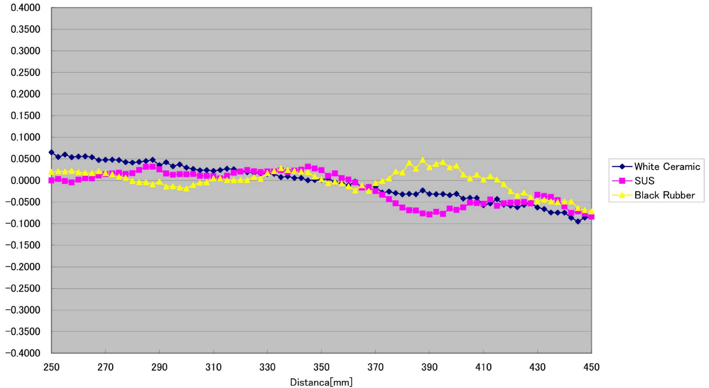
CD5-350-WIDE-800u Linearity(Horizontal 10° )[%FS] (Typical)
