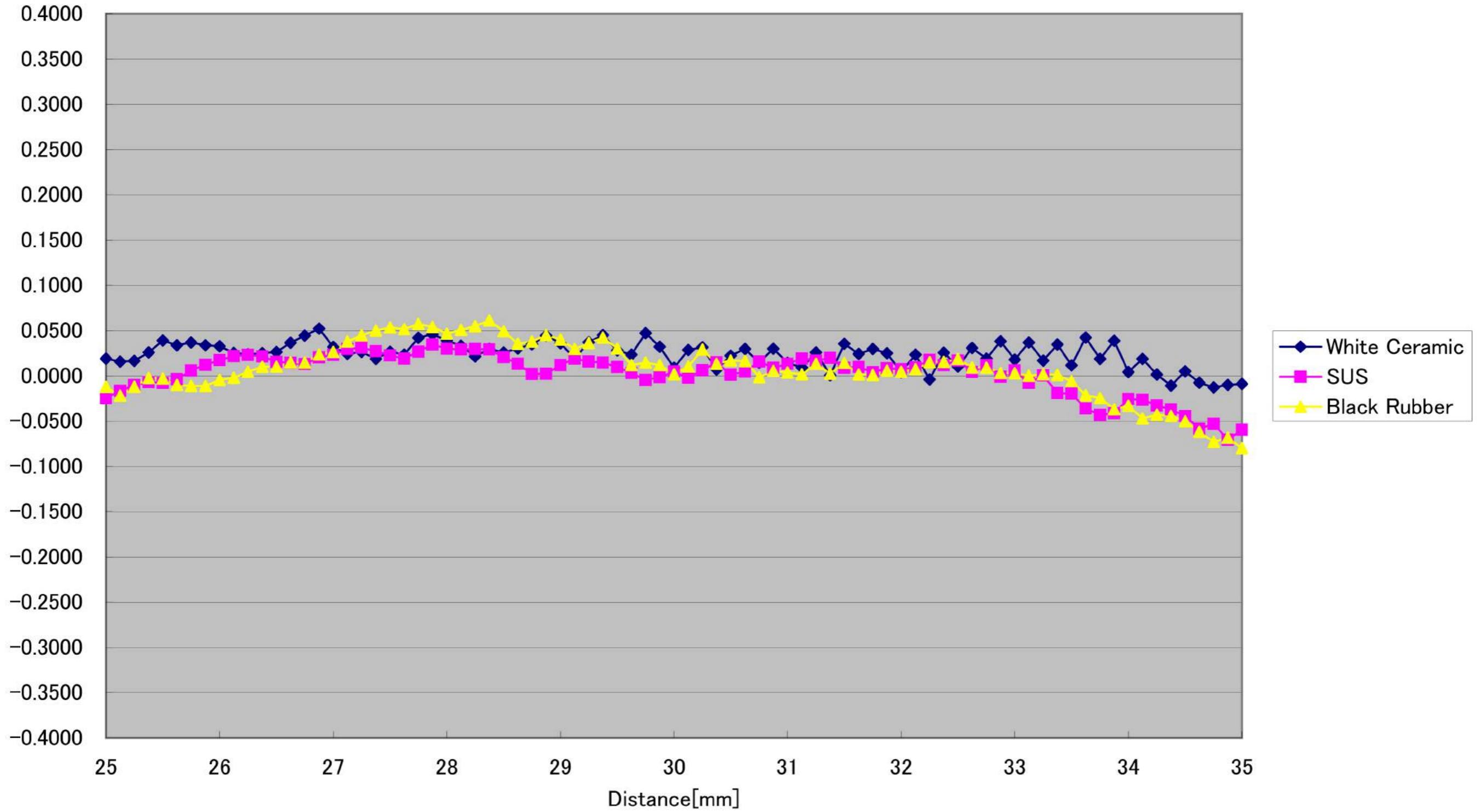
CD5-30-WIDE Linearity(Horizontal 10° )[%FS] (Typical)
