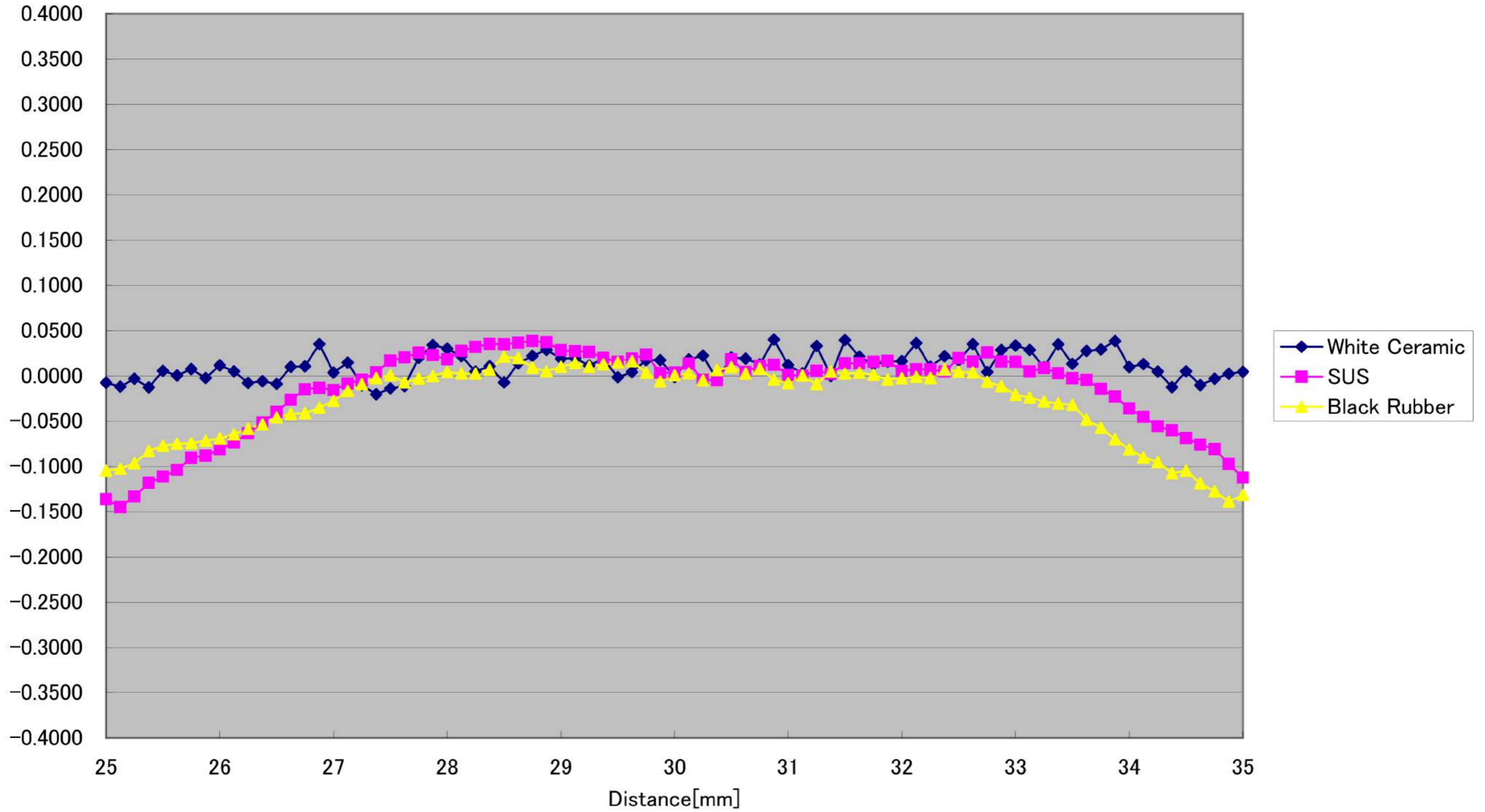
CD5-30-WIDE Linearity( \pm 0^\circ ) [%FS] (Typical)
