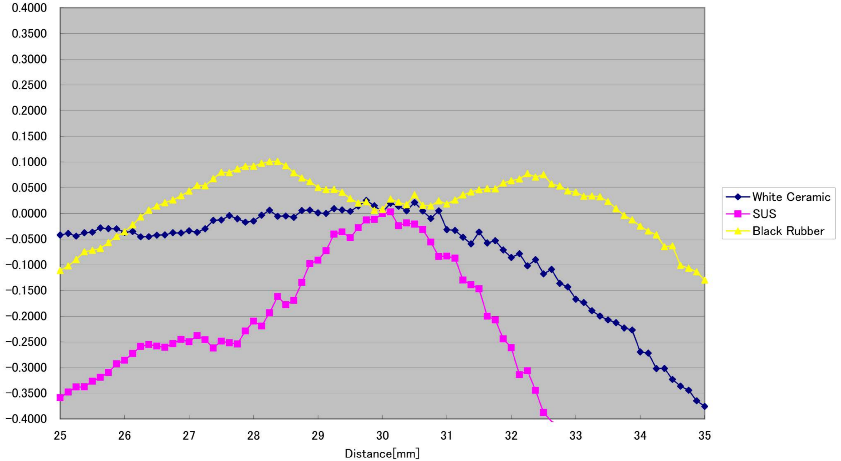
CD5-30-WIDE Linearity(Vertical +10° )[%FS] (Typical)
