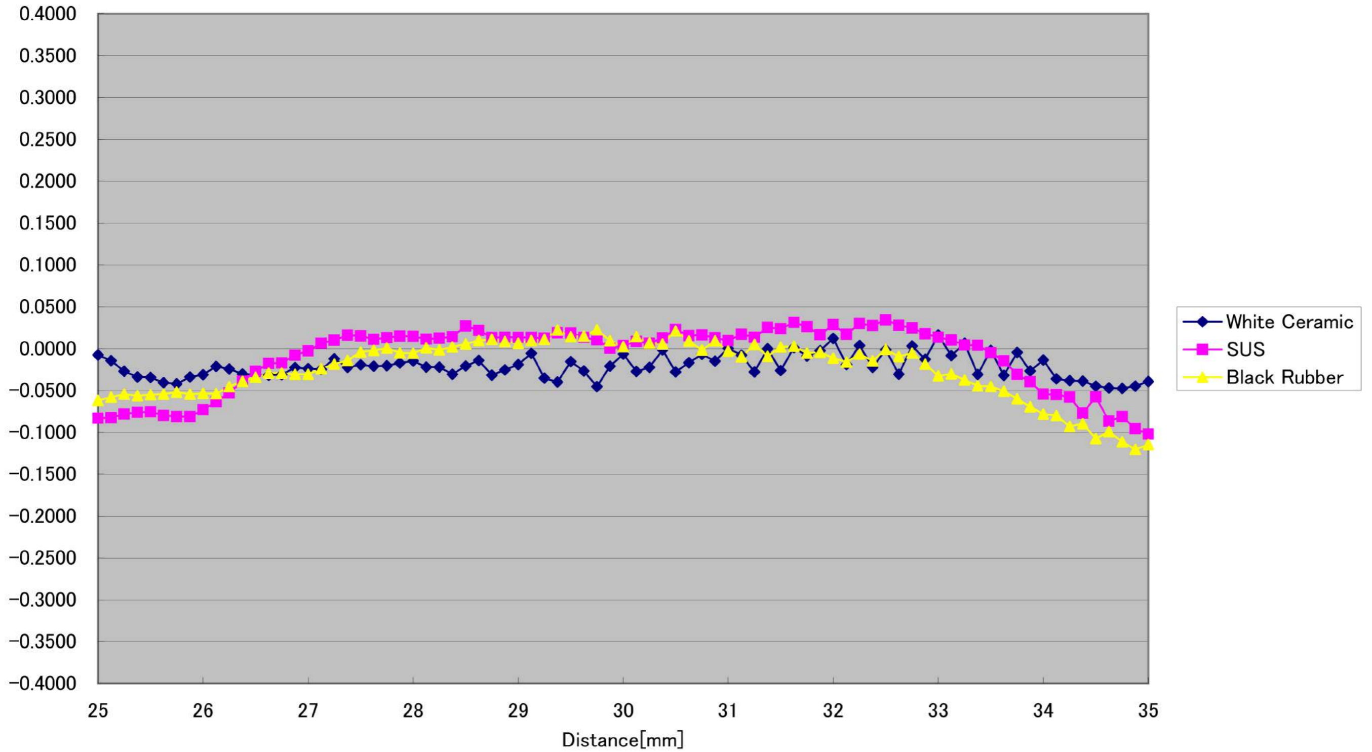
CD5-30-WIDE Linearity(Vertical -10^\circ )[%FS] (Typical)
