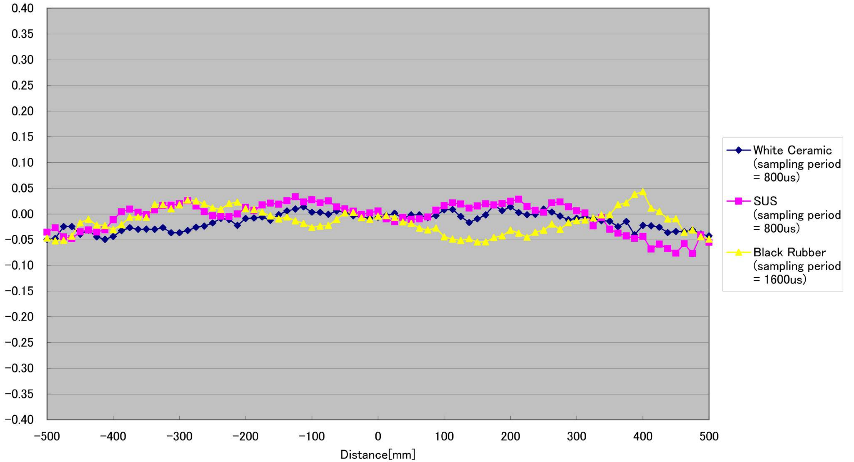
CD5-W2000 Linearity (Vertical +10° )[%FS]
