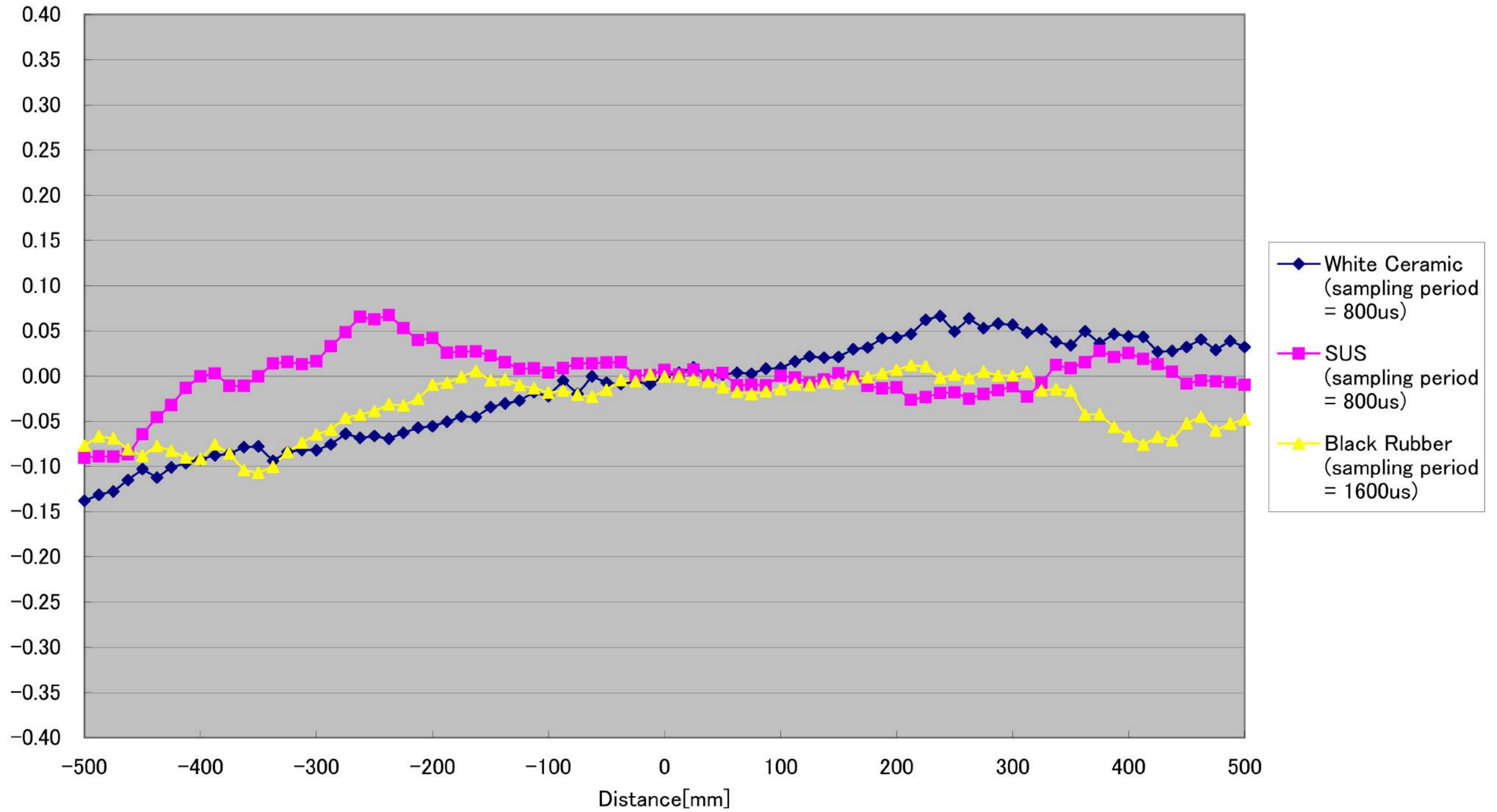
CD5-W2000 Linearity (Horizontal 10° )[%FS]
