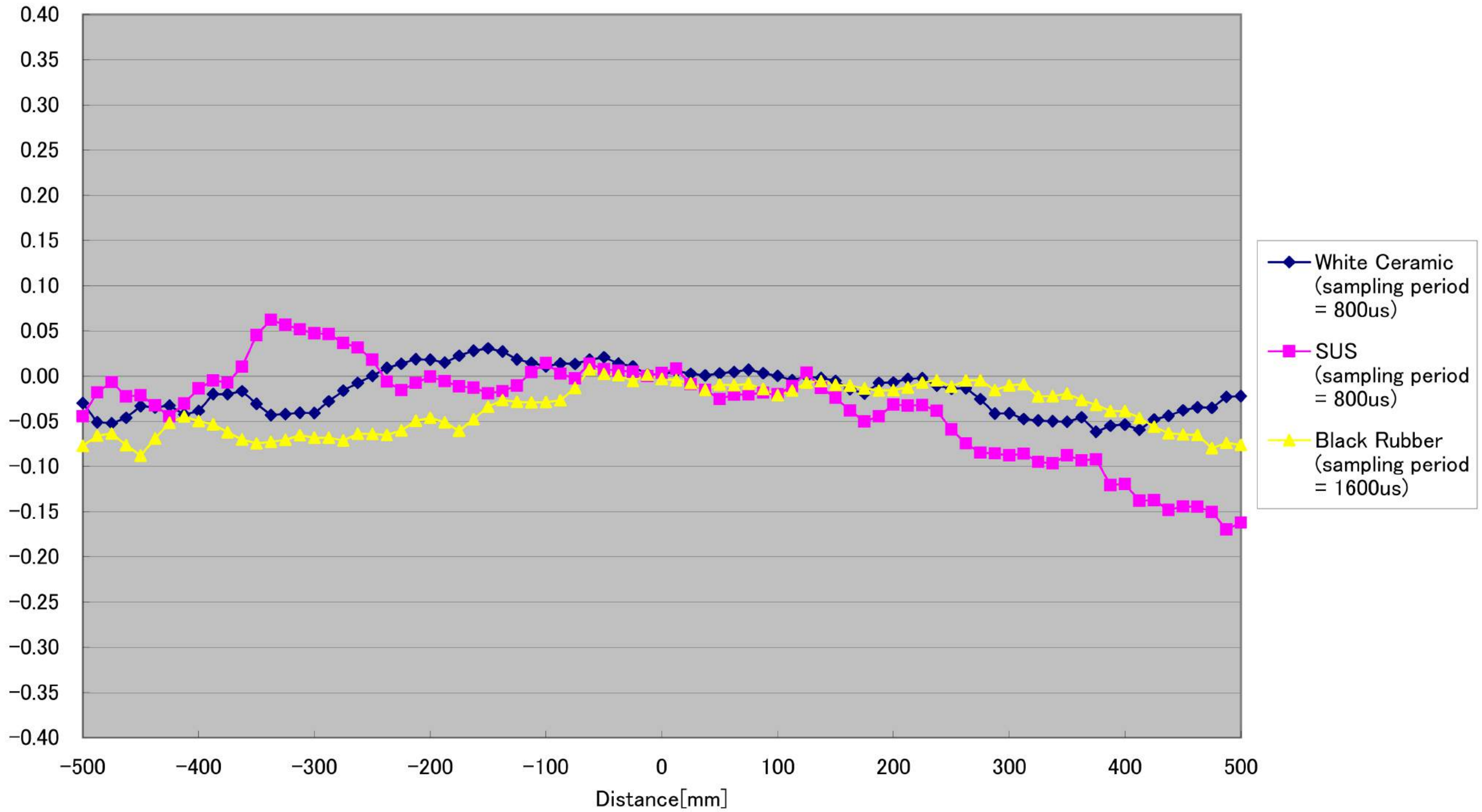
CD5-W2000 Linearity ( \pm 0^\circ ) [%FS]
