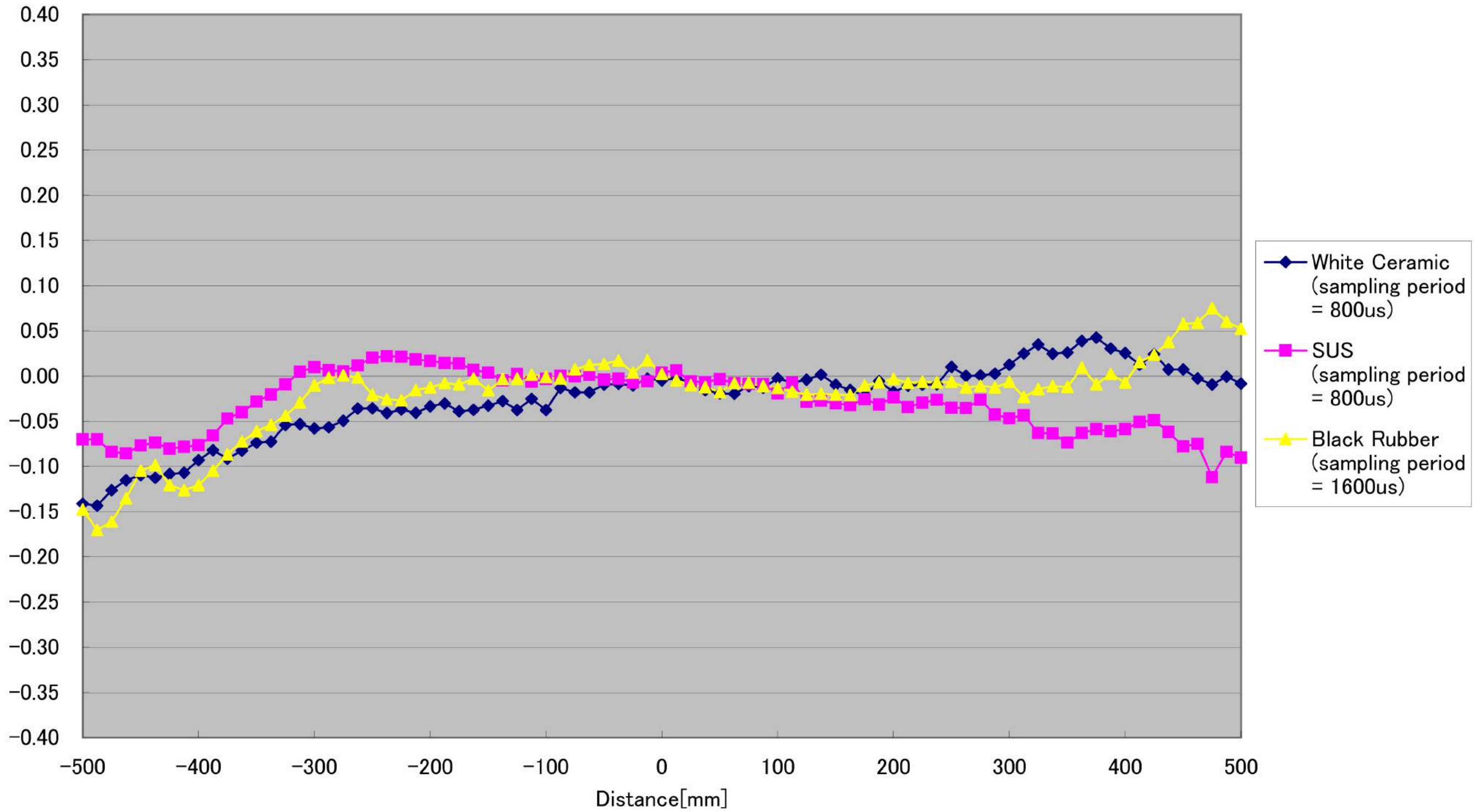
CD5-W2000 Linearity (Vertical -10^\circ ) [%FS]
