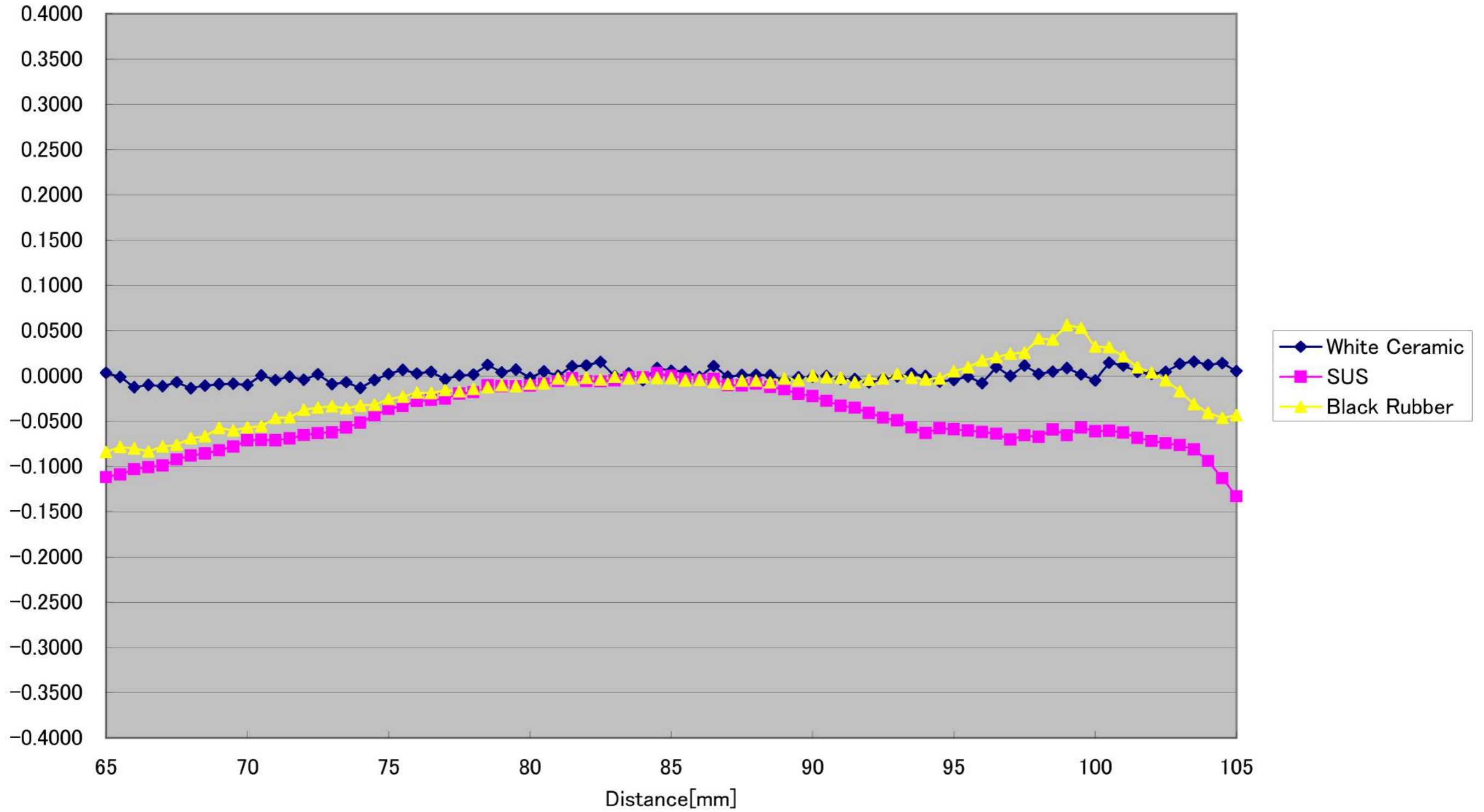
CD5-85-SPOT Linearity( \pm 0^\circ )[%FS] (Typical)
