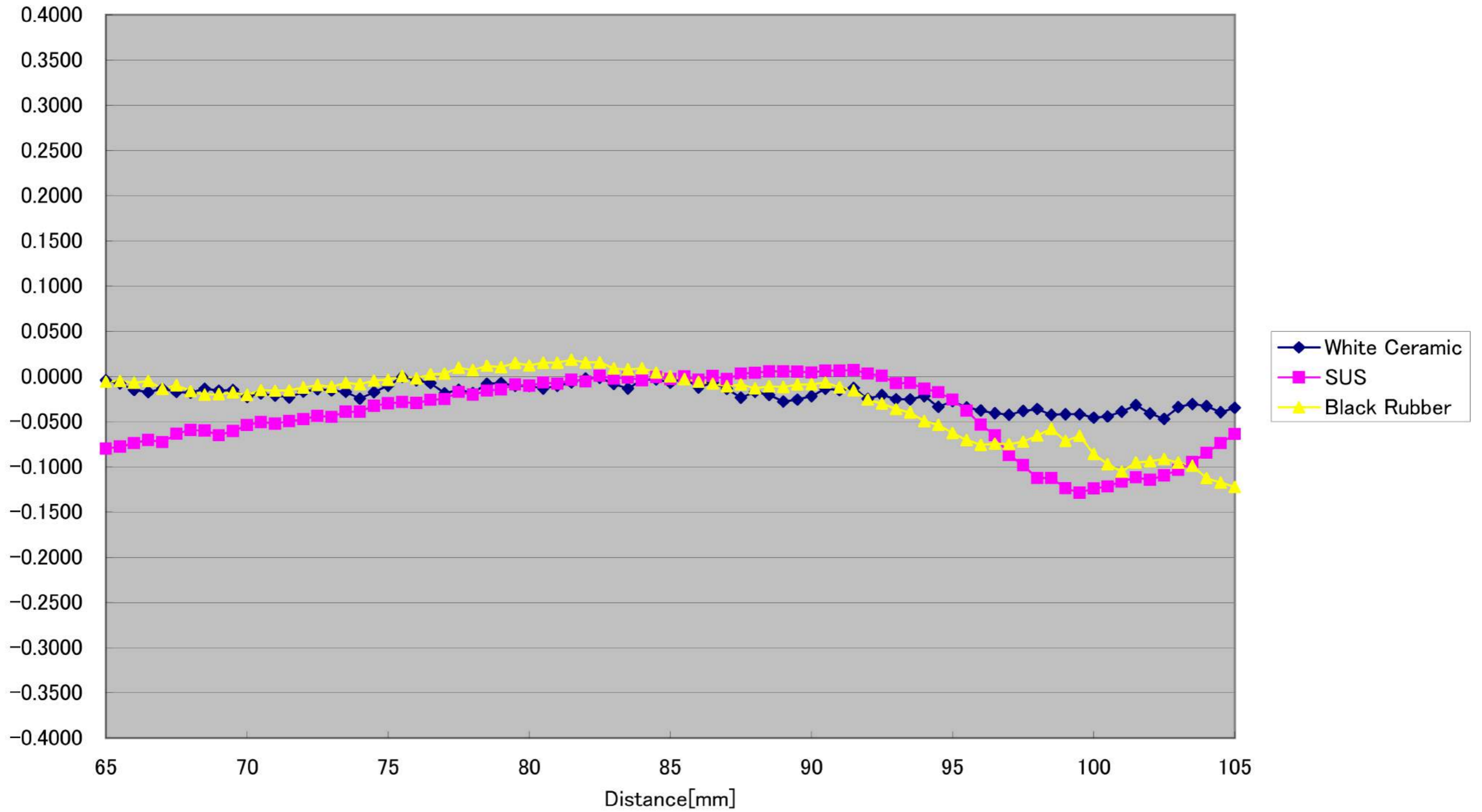
CD5-85-SPOT Linearity(Horizontal 10° )[%FS] (Typical)
