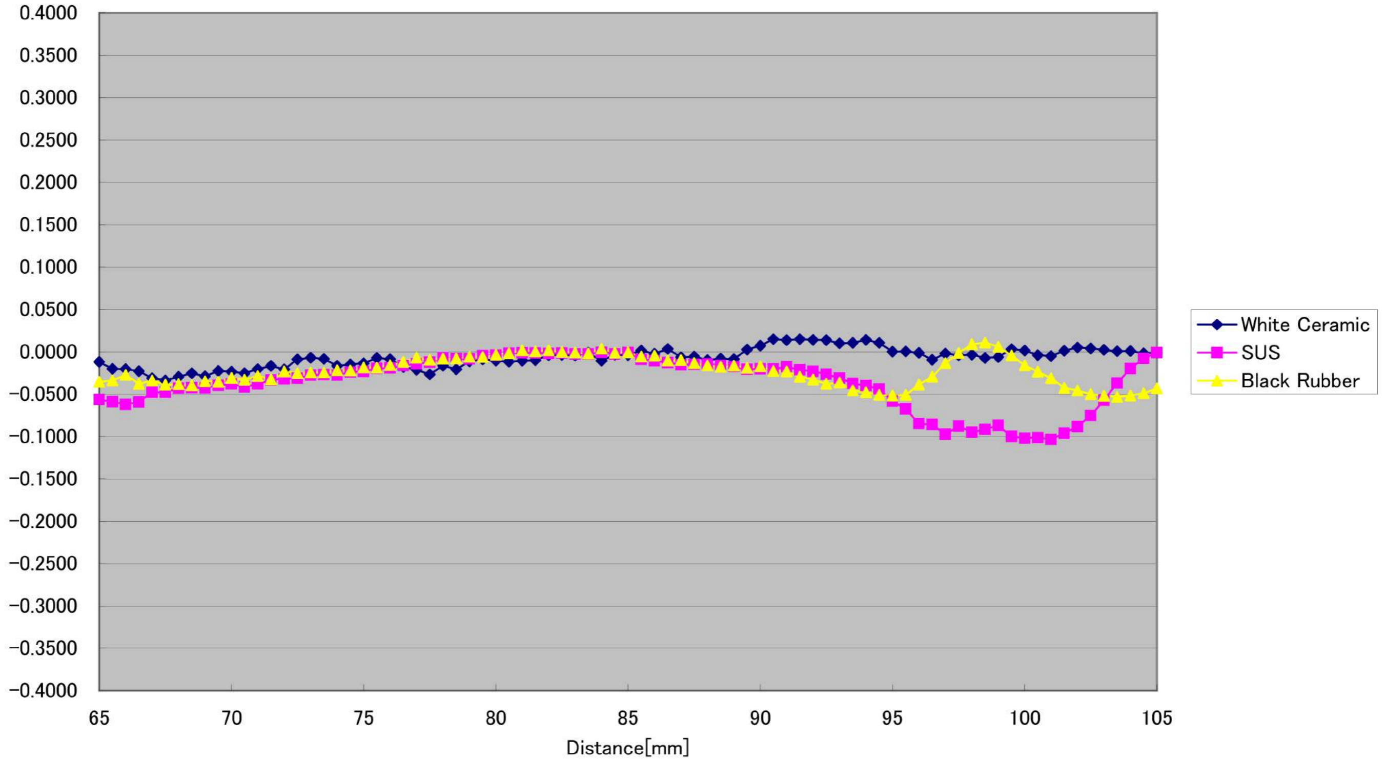
CD5-85-SPOT Linearity(Vertical -10° )[%FS] (Typical)
