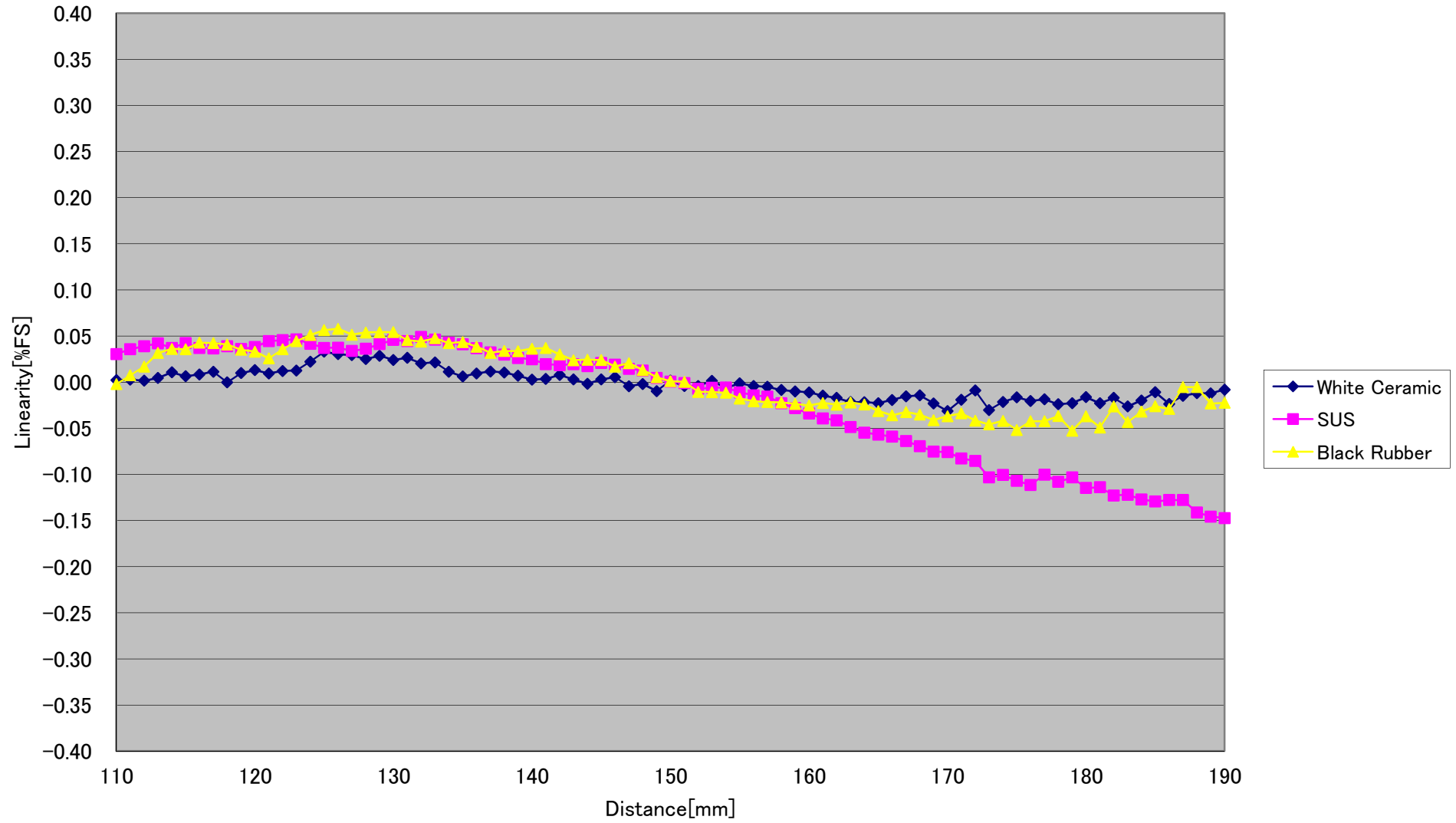
CD5-W150 Linearity(Vertical +10° )[%FS] (Typical)
