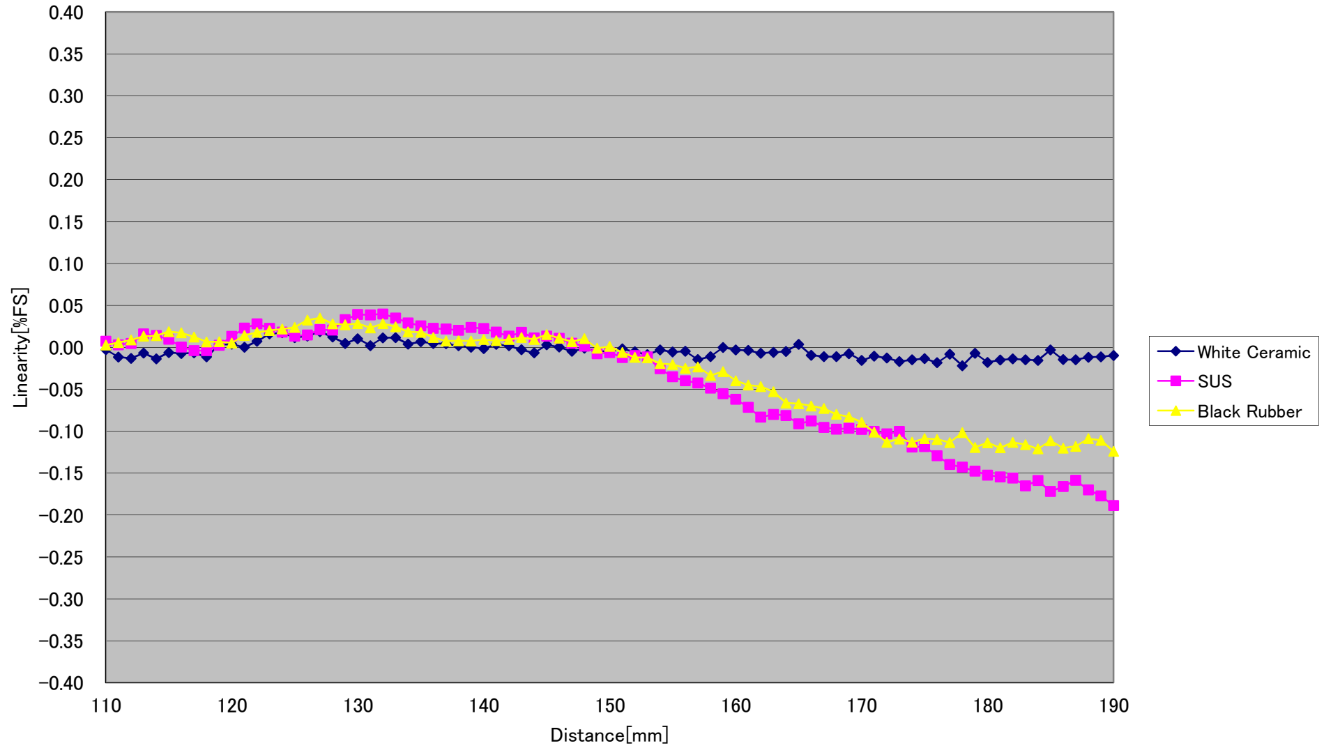
CD5-W150 Linearity( \pm 0^\circ )[%FS](Typical)
