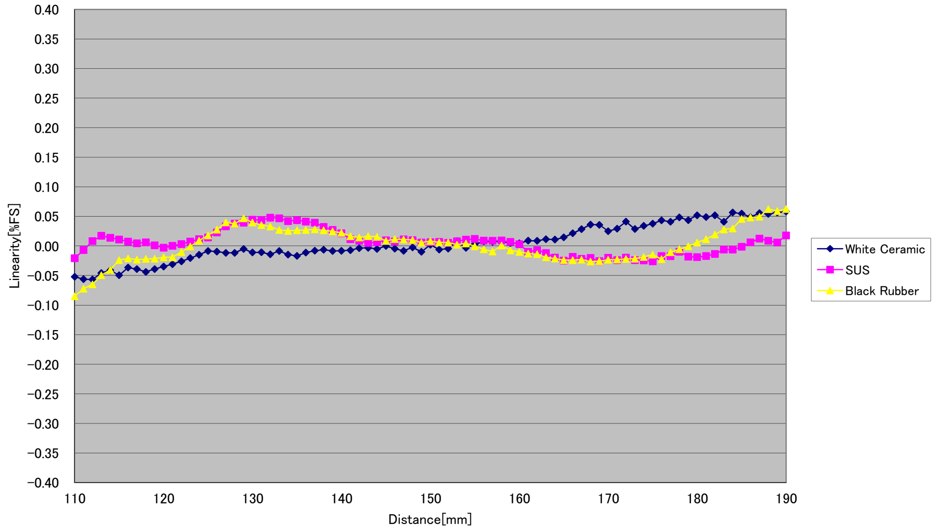
CD5-W150 Linearity(Horizontal 10° )[%FS] (Typical)
