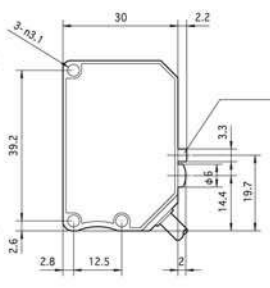
Cable type sensor
