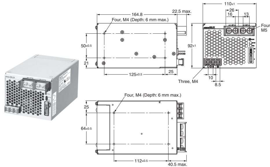
Panel mounting holes dimensions
