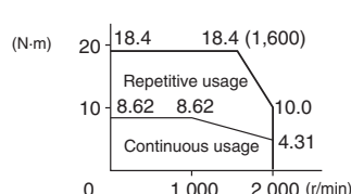
R88M-G90010T (900 W)
