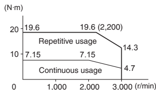
R88M-G1K520T (1.5 kW)
