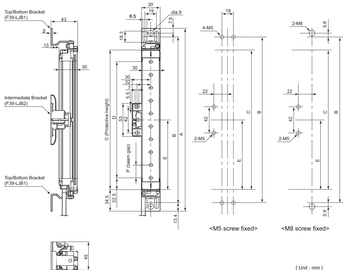
Dimensions A to E and P
