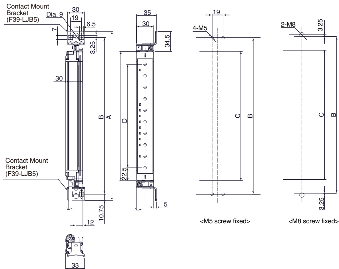
Dimensions A to D
