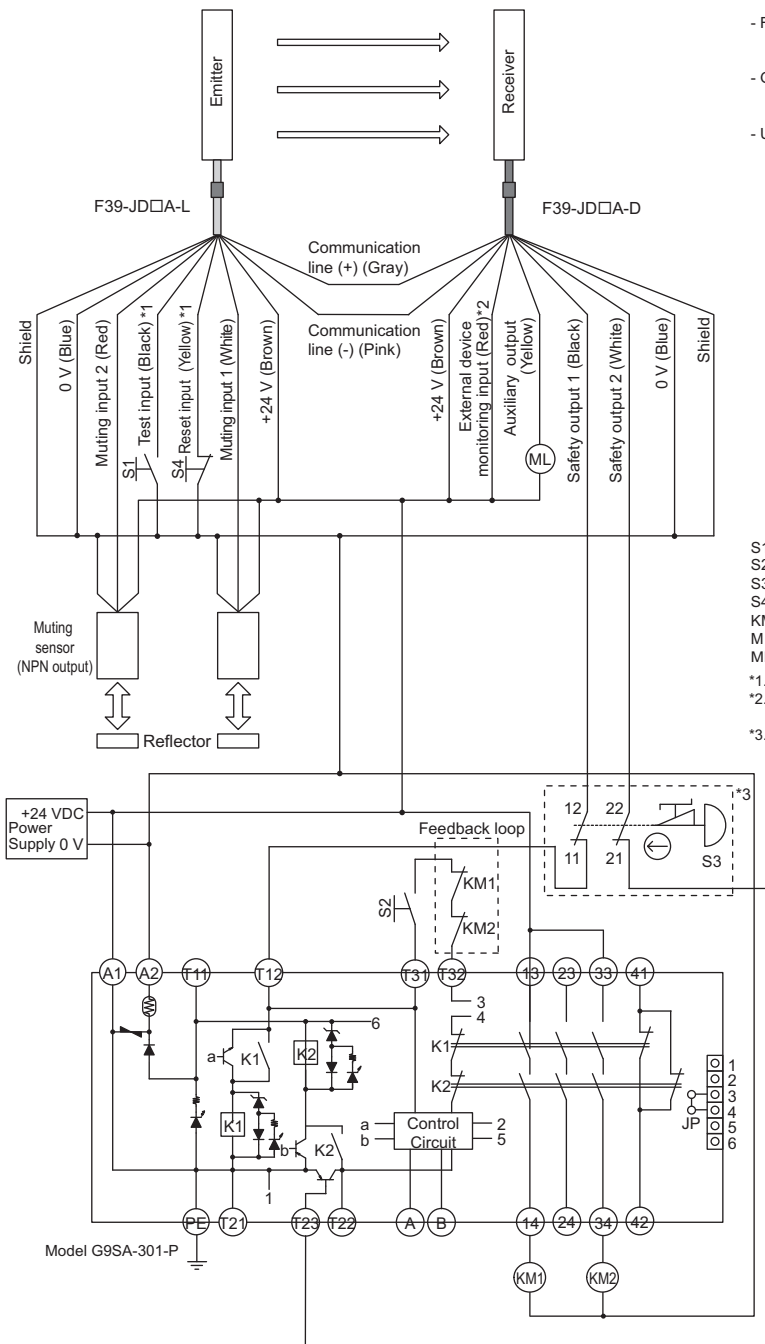
Wiring for auto reset mode
