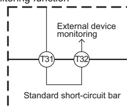
Wiring when not using external device monitoring function
