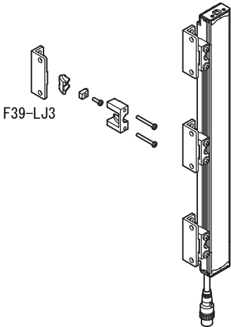
Backside mounting
