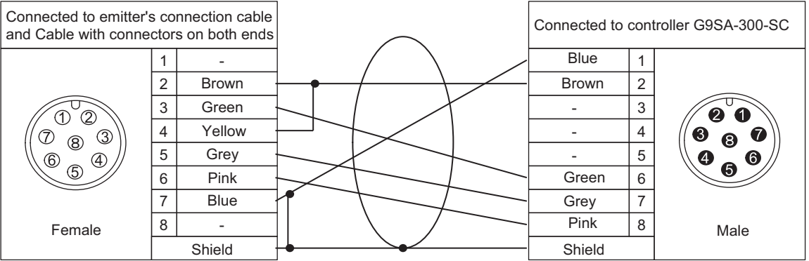
Internal wiring diagram (F39-JC□C-D)
