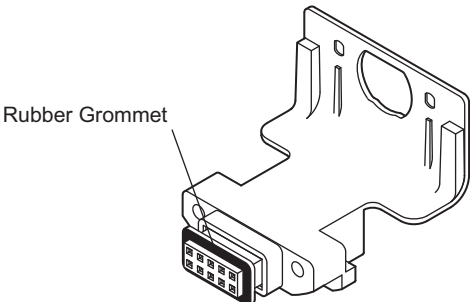
Misaligned Grommet
