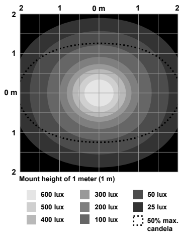
Figure 6. 1130 mm Models
