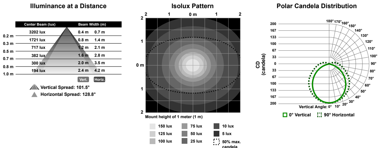
Figure 3. 285 mm Models
