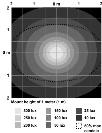
Figure 4. 570 mm Models
