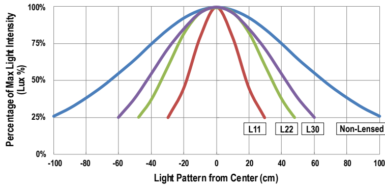
Figure 1. Percentage of Maximum Light Intensity for Lensed and Nonlensed Models at 1 Meter (Typical)
