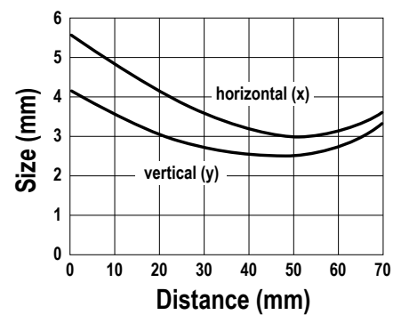
Adjustable Field Background Suppression
