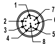
Euro-style Male Pinouts
